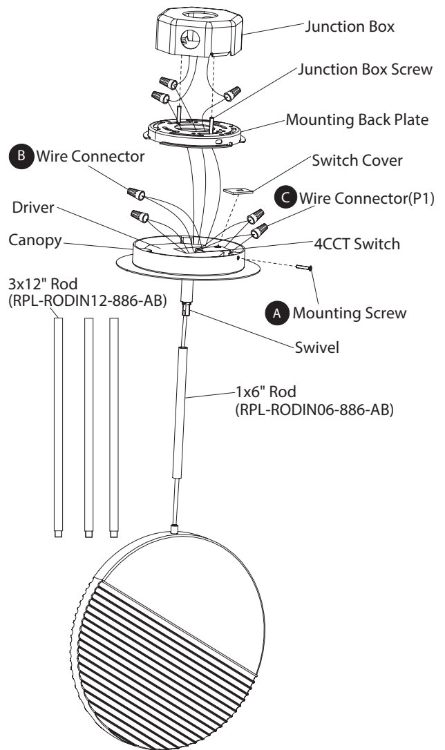
Fig. 6 Driver Wiring
